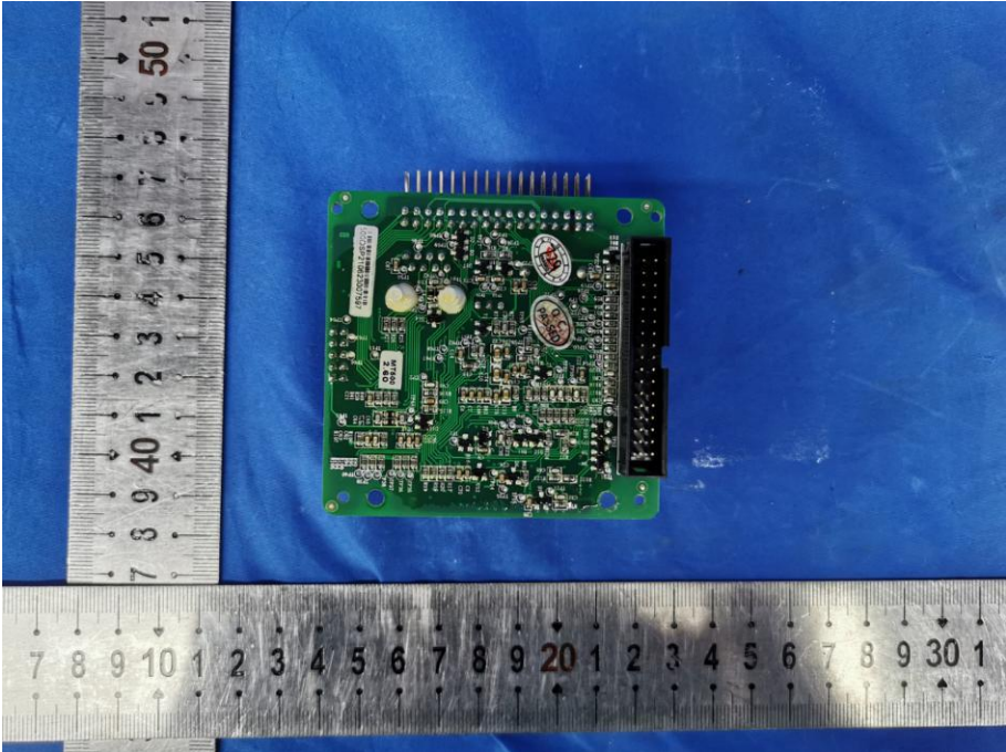
Fig. 12---PCB View
