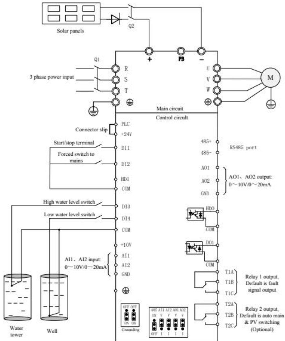
VFD500-PV Wire Diagram of solar pump inverter (three phase pump)
